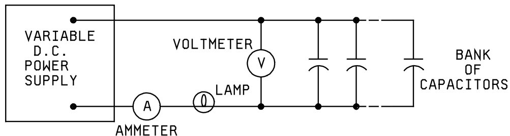
FIGURE 1. Schematic diagram.
